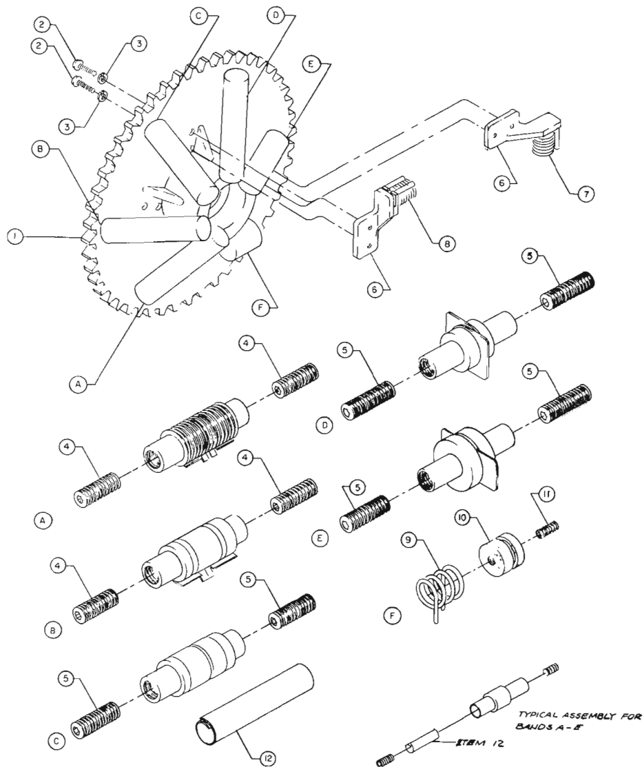
Figure 10. \phi Model 606A High Frequency Signal Generator, Oscillator Turret
