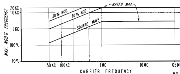
Figure 2-1. Modulating vs Carrier Frequency
