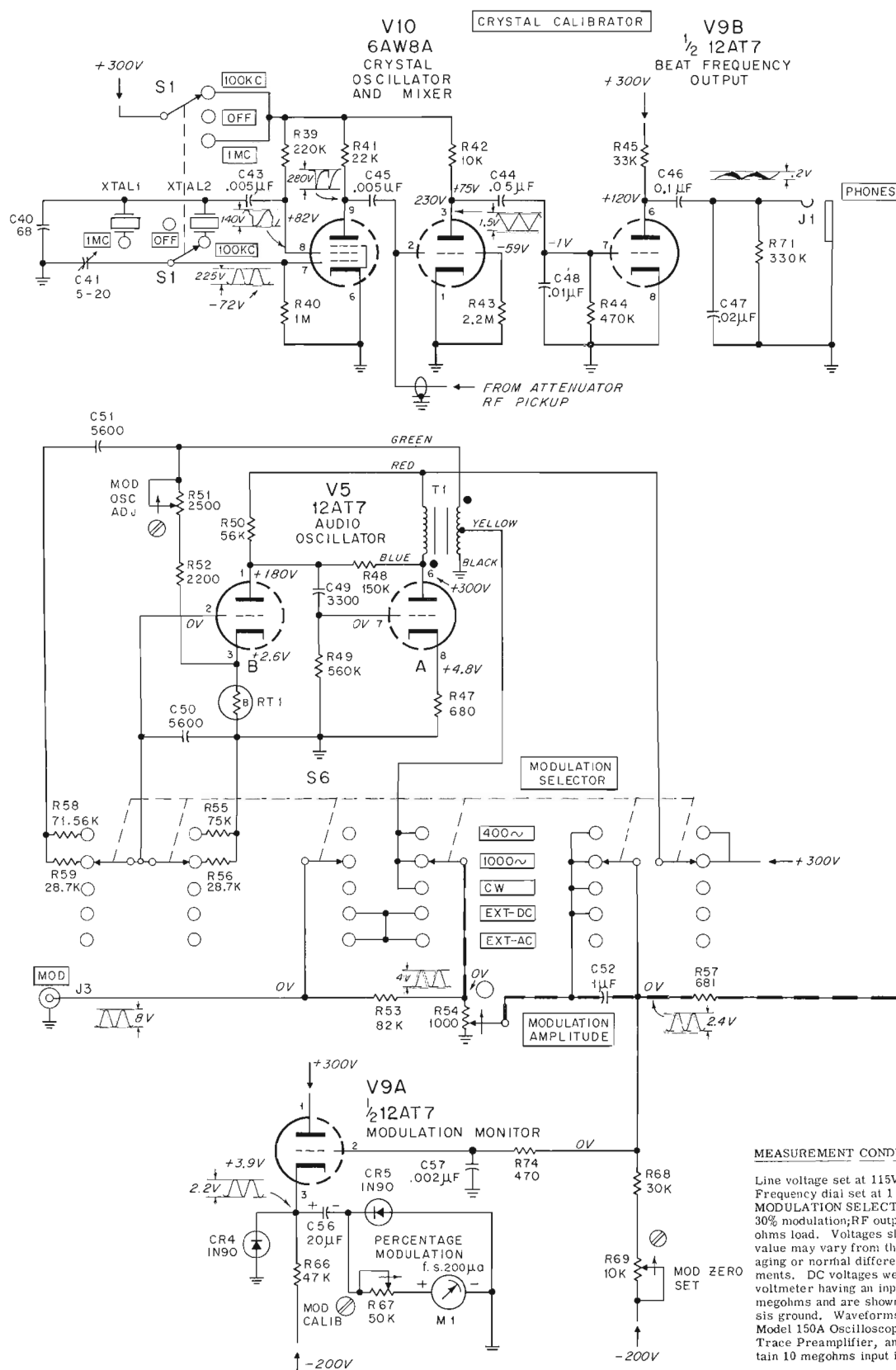
Figure 4-9. Signal Generator (Sheet 1 of 2)
